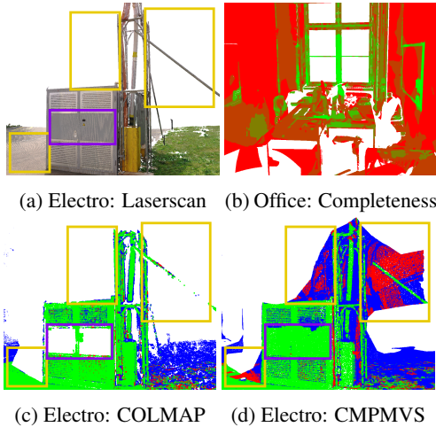
Figure 8. Qualitative results. See the text for details.
