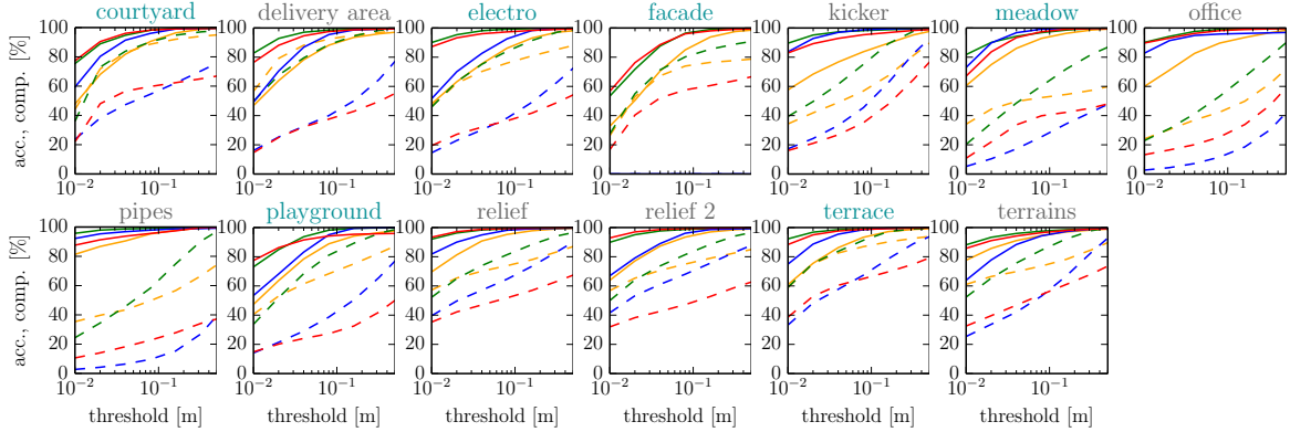
Figure 6. Evaluation of the high-resolution multi-view scenario (indoor and outdoor datasets). Results for CMPMVS, COLMAP, Gipuma, and PMVS are shown as a solid line for accuracy and as a dashed line for completeness.
